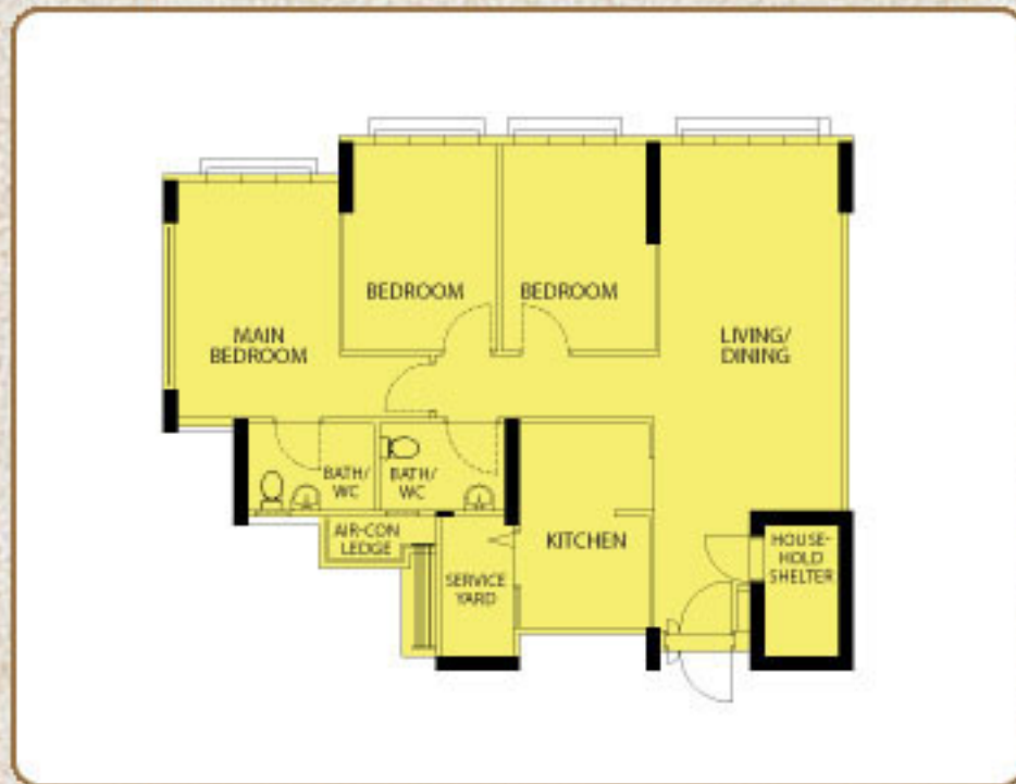
TYPICAL 4-ROOM FLOOR PLAN (WITH SINGULAR KITCHEN)
