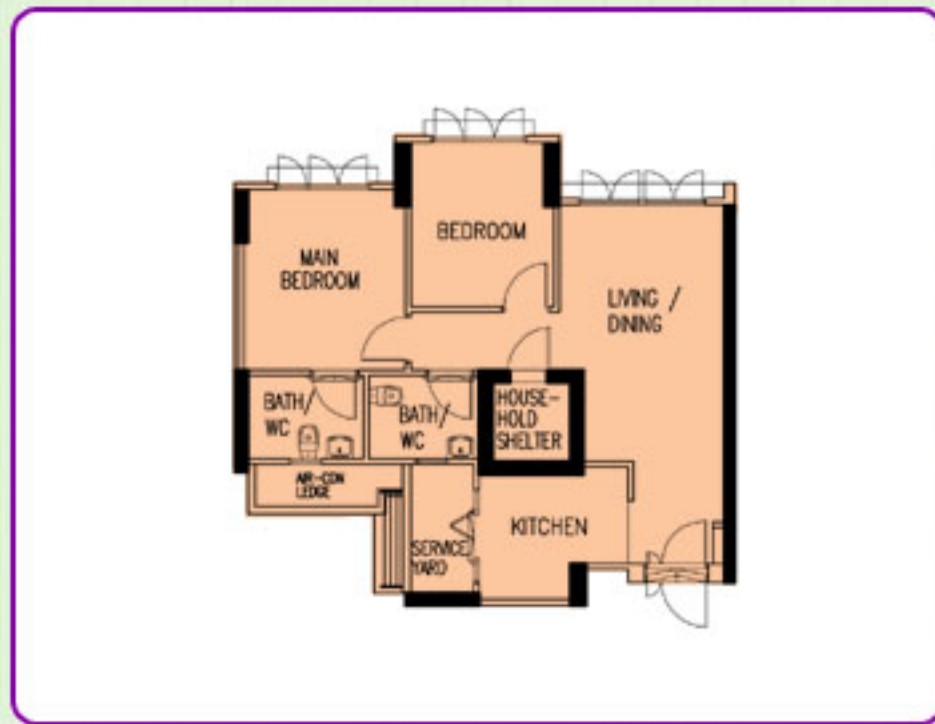
TYPICAL 3-ROOM FLOOR PLAN APPROX. FLOOR AREA 68 sqm
