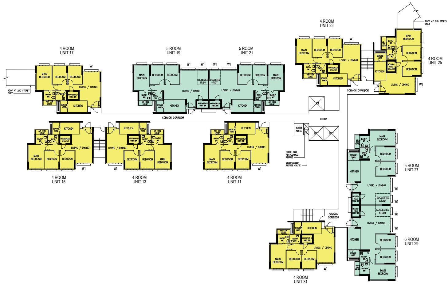
BLOCK 645A (2ND TO 11TH STOREY FLOOR PLAN)
